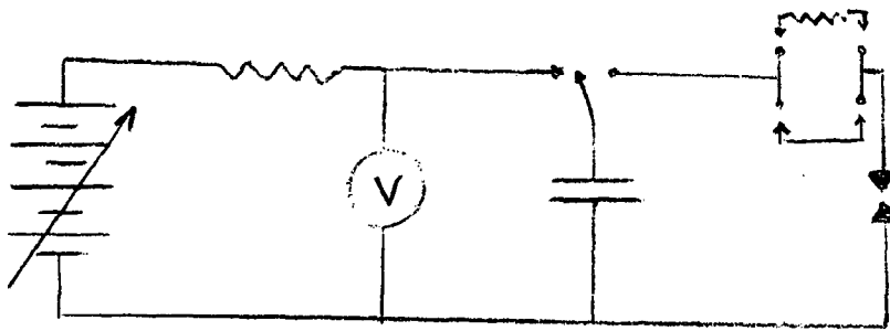
a Test Circuit
